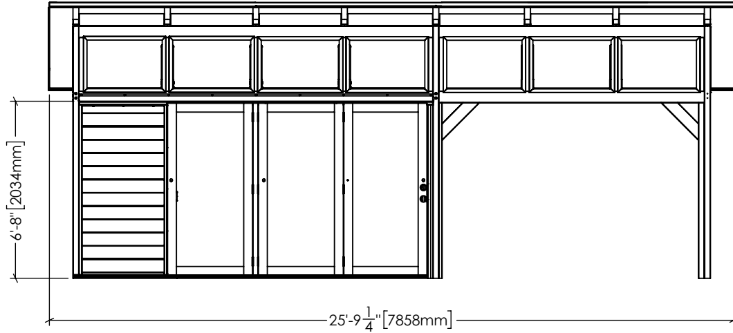
FRONT VIEW
